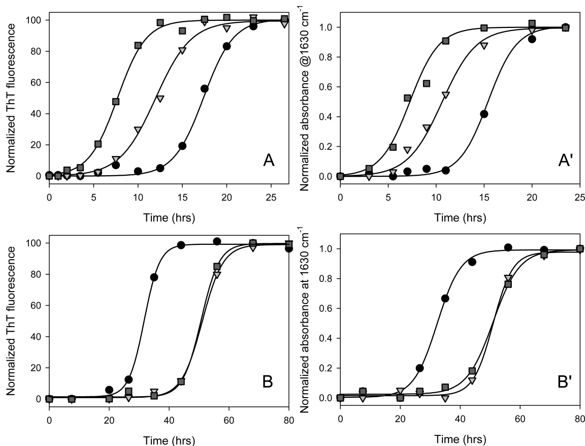
FIGURE 3: Fibrillation of human insulin in 20% acetic acid, pH 2.0 (A, A') or in 25 mM HEPES buffer, pH 7.5 (B, B') detected by changes in the ThT fluorescence intensity (plots A and B) and by the increase in the b-structure-related peak in the FTIR amide I spectrum (plots A' and B'). Protein (2 mg/mL) was incubated at 37 °C with stirring alone (circles) or in the presence of crowding agents: PEG-35080 (100 mg/mL, reversed triangles) and Ficoll-70000 (150 mg/mL, squares). At appropriate time points, small samples were taken for ThT or FTIR measurements.
