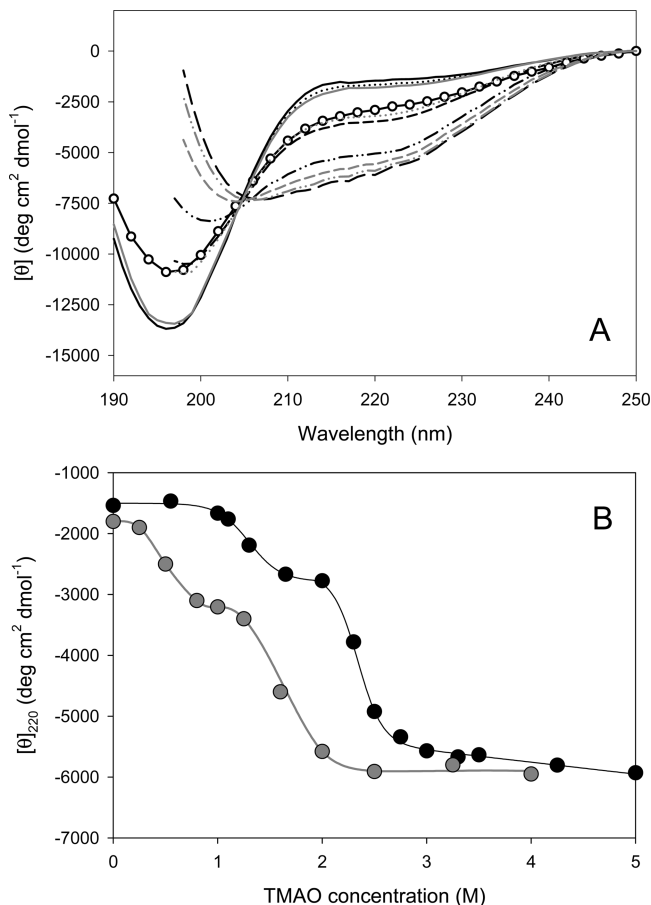
FIGURE 9: Effect of TMAO and Ficoll-70000 on structural properties of human \alpha -synuclein. (A) Far-UV CD spectra measured for 0.5 mg/mL \alpha -synuclein in the absence (dark lines) and presence (gray lines) of 150 mg/mL Ficoll-70000. Solid lines correspond to the protein in the absence of TMAO, whereas dotted, short dashed and dash-dotted lines represent data obtained in the presence of 1.0 M, 2.0 and 2.5 M TMAO, respectively. Black long dashed line corresponds to \alpha -synuclein in the presence of 4.5 M TMAO. Spectrum of the amyloidogenic partially folded conformation induced in \alpha -synuclein at acidic pH is shown as a line with open circles. (B) TMAO-induced changes in the [\theta]_{220} measured in the absence (black circles and black line) or in the presence of 150 mg/mL Ficoll-70000 (gray circles and gray line).
