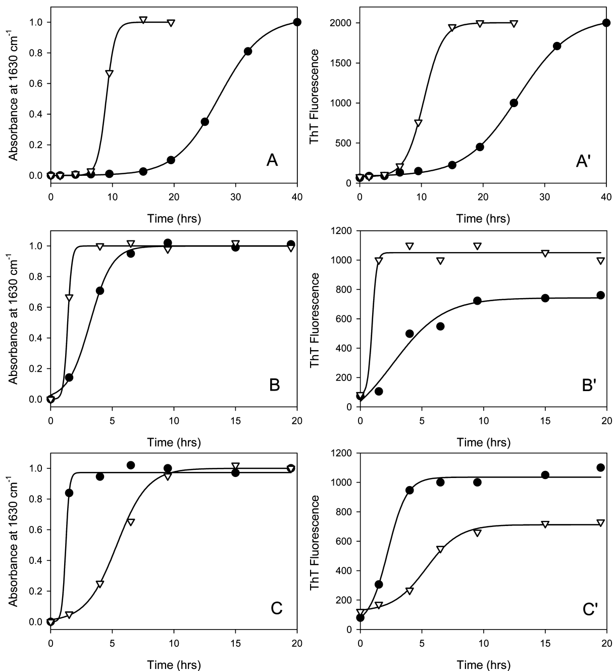
FIGURE 8: Fibrillation of human recombinant \alpha -synuclein in the absence (black circles) and the presence of 150 mg/mL Ficoll-70000 (open reversed triangles). Fibrillation was assessed by the increase in the intensity of the FTIR peak at 1630\text{ cm}^{-1} (plots A, B, and C) or via the characteristic increase in the ThT fluorescence (plots A', B', and C'). Protein (0.5 mg/mL) was incubated at 37^\circ\text{C} with stirring alone (circles) or in the presence of Ficoll-70000 (150 mg/mL, squares). Panels A and A' represent data at 0 M TMAO, panels B and B' were obtained in the presence of 1 M TMAO, whereas panels C and C' show data for 2 M TMAO. At appropriate time points, small samples were taken for ThT or FTIR measurements.
