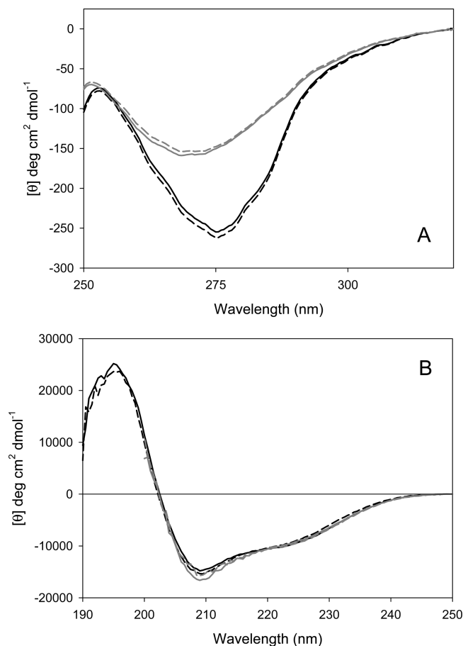
FIGURE 4: Effect of macromolecular crowding agent Ficoll-70000 (150 mg/mL, dashed lines) on near-UV CD (A) and far-UV CD spectra of human insulin (B) in different conformational states: native hexameric protein in 25 mM HEPES buffer, pH 7.5 (black lines) and in 20% acetic acid, pH 2.0 (gray lines). Solid lines in both plots correspond to spectra measured in the absence of the crowder.
