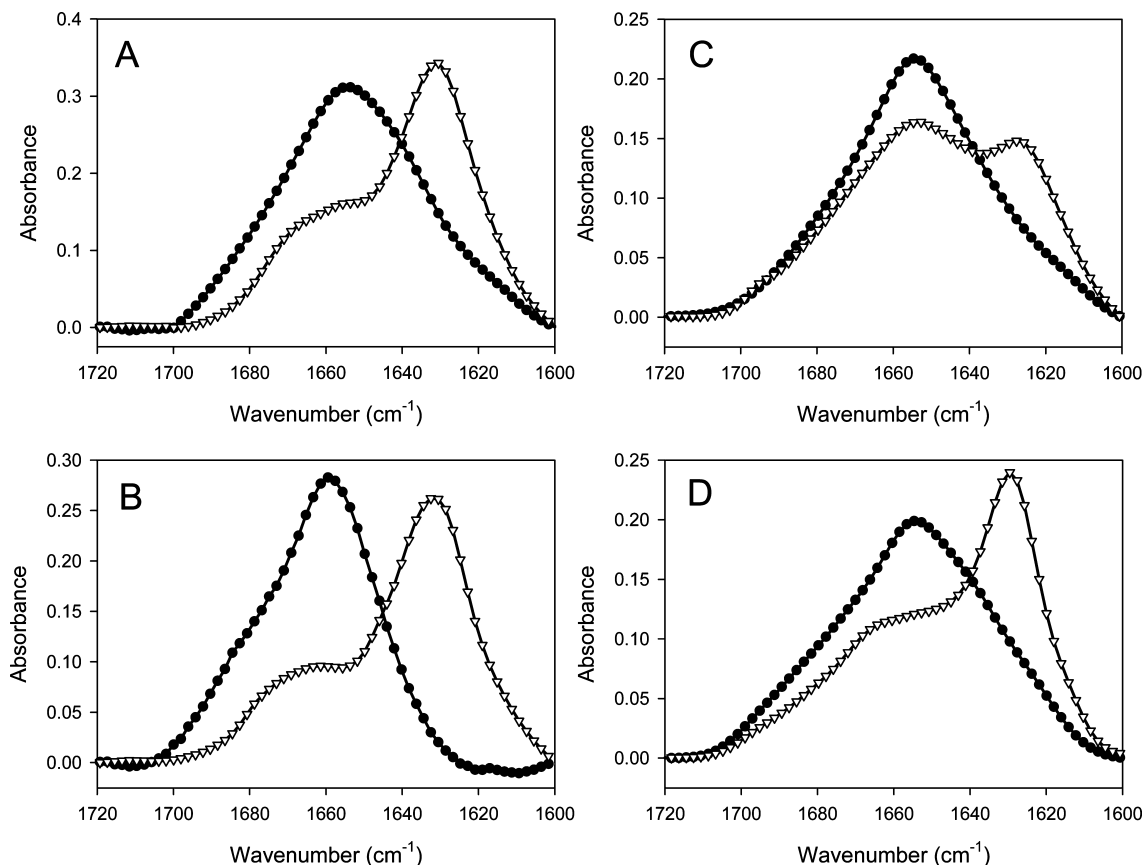
FIGURE 1: FTIR amide I spectra of bovine S -carboxymethyl- \alpha -lactalbumin (A), human insulin (B), bovine core histones (C) and human \alpha -synuclein (D) in nonfibrillar (black circles) and fibrillar forms after the incubation at appropriate conditions at 37 °C with stirring (open reversed triangles).
