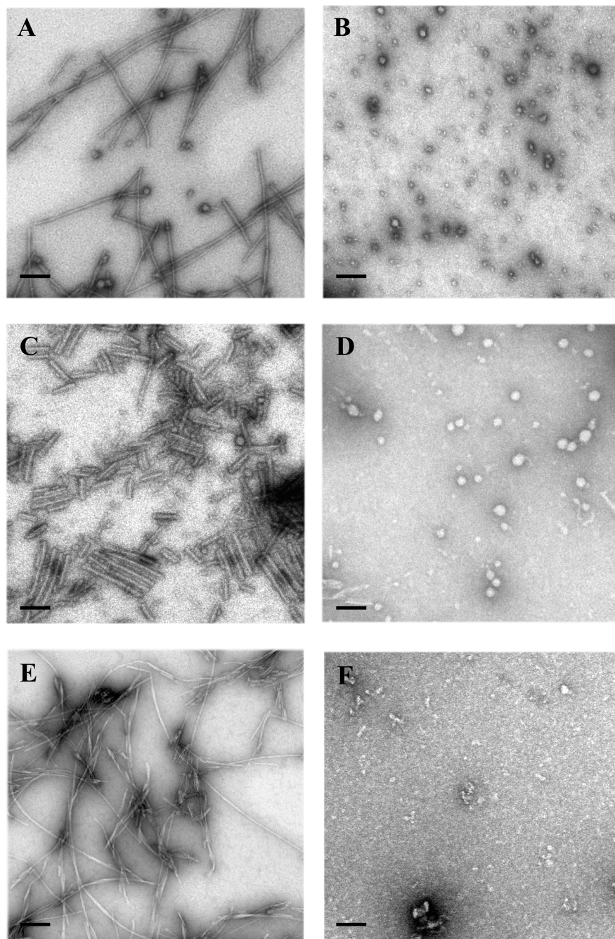
FIGURE 5: EM of insulin, \alpha -synuclein, and histone aggregates. (A) Fibrils of \alpha -synuclein grown in the presence of Ficoll-70000 and 1 M TMAO (5 h of incubation); (B) oligomers of \alpha -synuclein formed in the presence of Ficoll-70000 and 2.5 M TMAO (5 h of incubation); (C) fibrils of histones grown at pH 2.0 and PEG 10,000 (48 h of incubation); (D) oligomers and amorphous aggregates of histones formed at pH 7.5 and PEG 10,000 (48 h of incubation); (E) insulin fibrils grown at pH 2 and PEG 10,000 (20 h of incubation); (F) oligomers and amorphous aggregates of insulin formed at pH 7.5 and PEG 10,000 (20 h of incubation). Scale bar is 100 nm.
