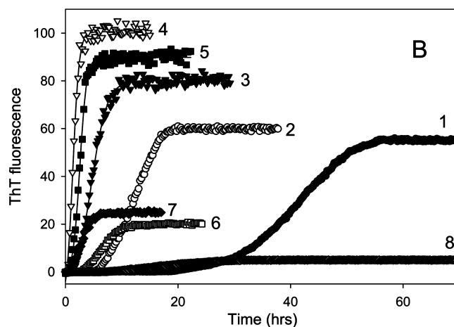
FIGURE 7: Fibrillation of human recombinant \alpha -synuclein in the absence (black symbols) or presence of 100 mg/mL PEG-3500 (open symbols). Protein was incubated alone (circles) or in the presence of 1 (reversed triangles), 2 (squares) or 2.5 M TMAO (diamonds). Panel A represents a set of normalized data, whereas panel B shows the same data in the non-normalized form. In panel B numbers correspond to (1) control, no additives; (2) \alpha -synuclein + PEG; (3) 1 M TMAO; (4) 1 M TMAO + PEG; (5) 2 M TMAO; (6) 2 M TMAO + PEG; (7) 2.5 M TMAO; (8) 2.5 M TMAO + PEG. Protein at a concentration of 0.5 mg/mL was incubated in 20 mM Tris-HCl, 100 mM NaCl buffer pH 7.5 at 37 °C with agitation, and fibrillation was monitored by the enhancement of thioflavin T fluorescence intensity.
