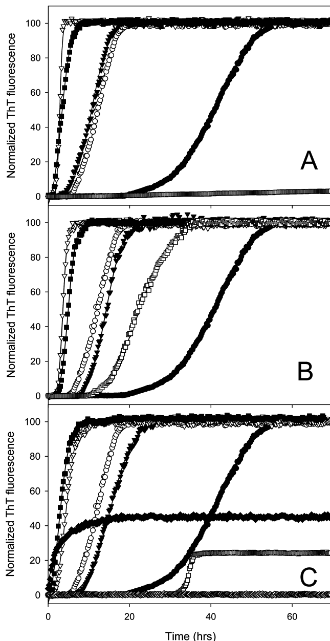
FIGURE 10: Effects of different alcohols on the fibrillation of \alpha -synuclein in the absence (black symbols) or presence of 100 mg/mL PEG-3500 (open symbols). Fibrillation was monitored by Thioflavin T. \alpha -Synuclein (0.5 mg/mL) was incubated at 37 °C with agitation in the various aqueous–organic solvents. (A) EtOH; (B) TFE; (C) HFiP. EtOH concentrations were 0% ( \circ ), 10% ( \nabla ), and 20% ( \square ). TFE concentrations were 0% ( \circ ), 5% ( \nabla ), and 10% ( \square ). HFiP concentrations were 0% ( \circ ), 1% ( \nabla ), 2.5% ( \square ) and 5% ( \diamond ).
