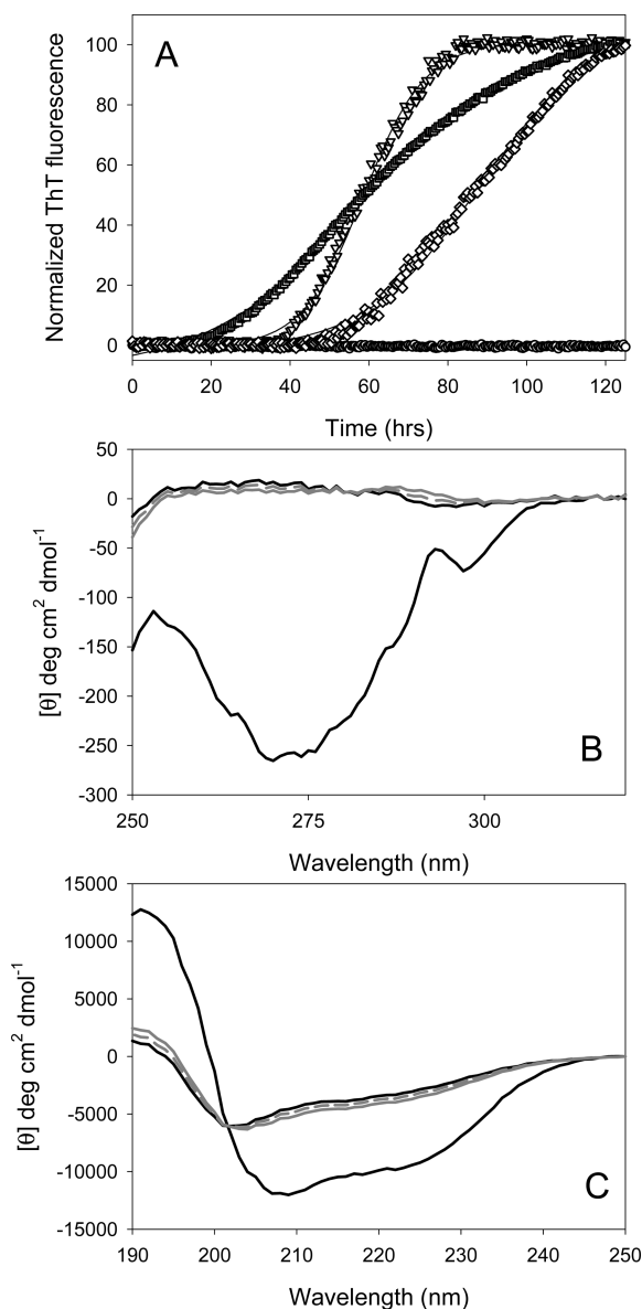
FIGURE 2: Effect of crowding agents on fibrillation and structural properties of bovine S -carboxymethyl- \alpha -lactalbumin. (A) Fibrillation of bovine S -carboxymethyl- \alpha -lactalbumin (1 mg/mL) monitored by the enhancement of thioflavin T fluorescence intensity at 37 °C with stirring in the absence (circles) or presence of high concentrations of model macromolecular crowding agents: PEG-3500 (100 mg/mL, reversed triangles), Ficoll-70000 (150 mg/mL, diamonds) and bovine serum albumin (30 mg/mL, squares). Conditions were 20 mM Tris-HCl, 100 mM NaCl, pH 7.5. (B) Near-UV CD spectra of the native \alpha -lactalbumin (solid black line 1) and its S -carboxymethylated form (solid black line 2) in the absence of crowding agents, as well as in the presence of PEG-3500 (100 mg/mL, solid gray line) and Ficoll-70000 (150 mg/mL, dashed gray line). (C) Far-UV CD spectra of the native (solid black line 1) and its S -carboxymethyl- \alpha -lactalbumin (solid black line 2) in the absence of crowding agents, as well as in the presence of PEG-3500 (100 mg/mL, solid gray line) and Ficoll-70000 (150 mg/mL, dashed gray line).
